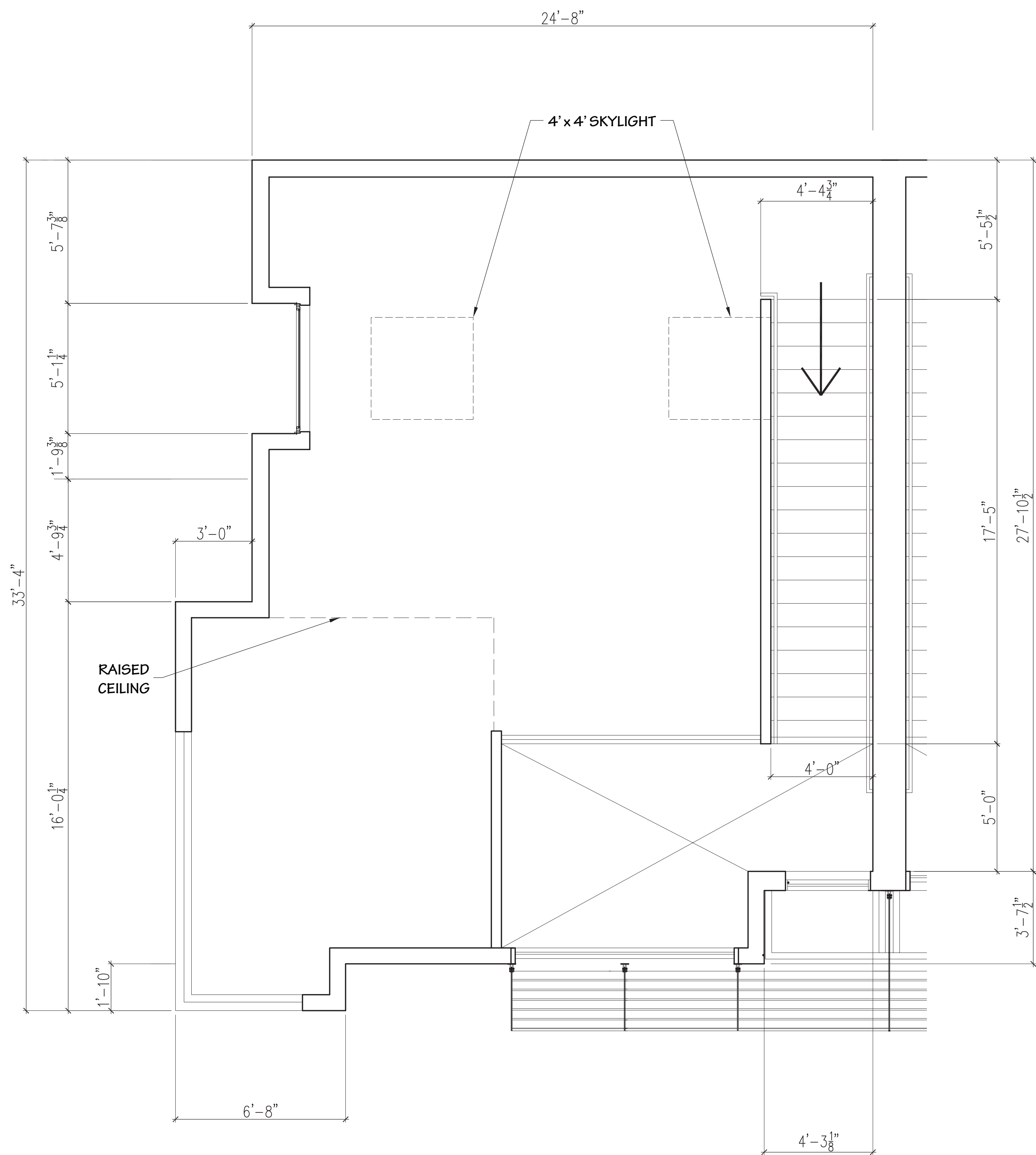
2 Unit A 2nd Floor Plan 3/8" = 1'-0"
