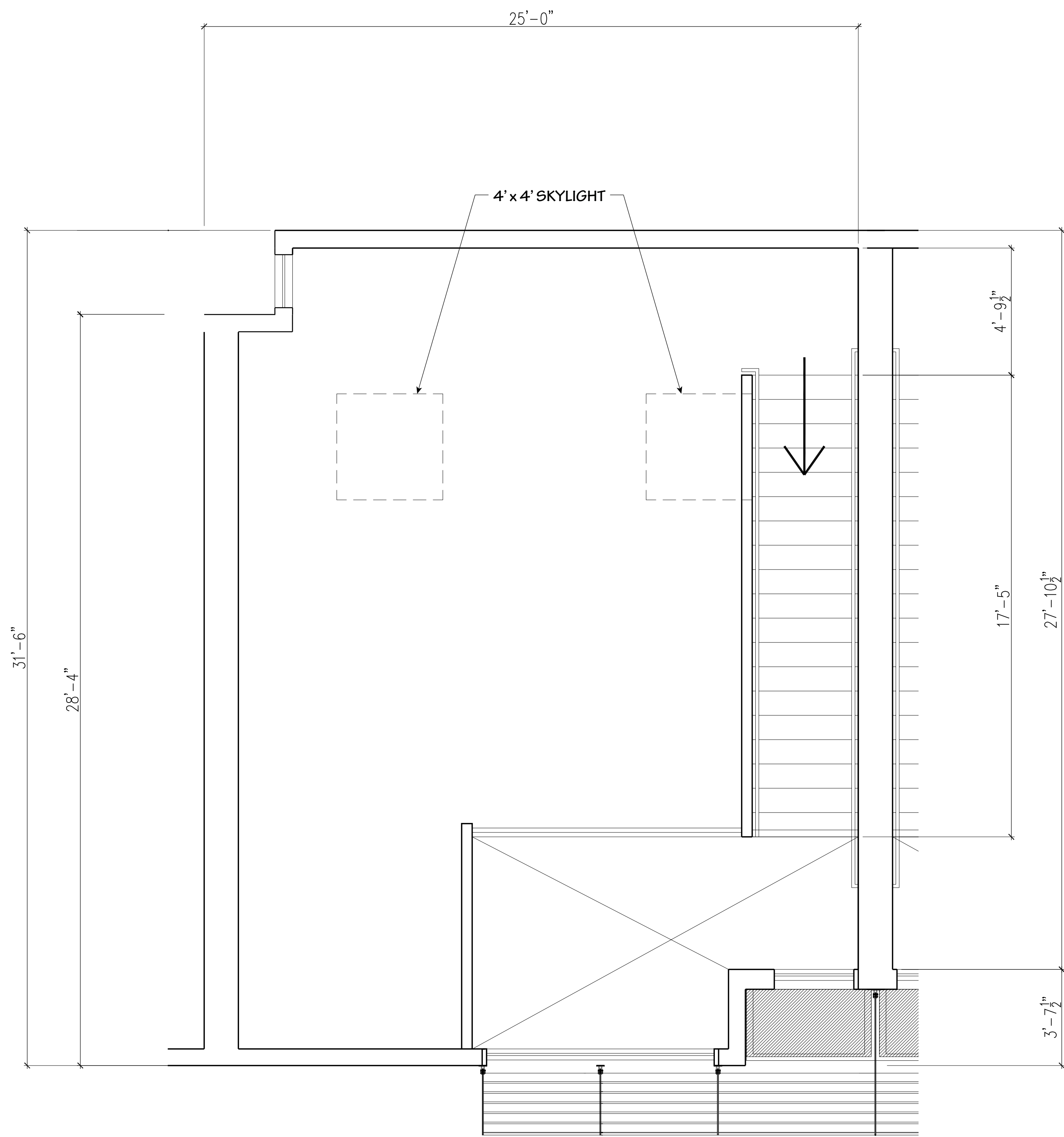
2 Unit C 2nd Floor Plan 3/8" = 1'-0"
