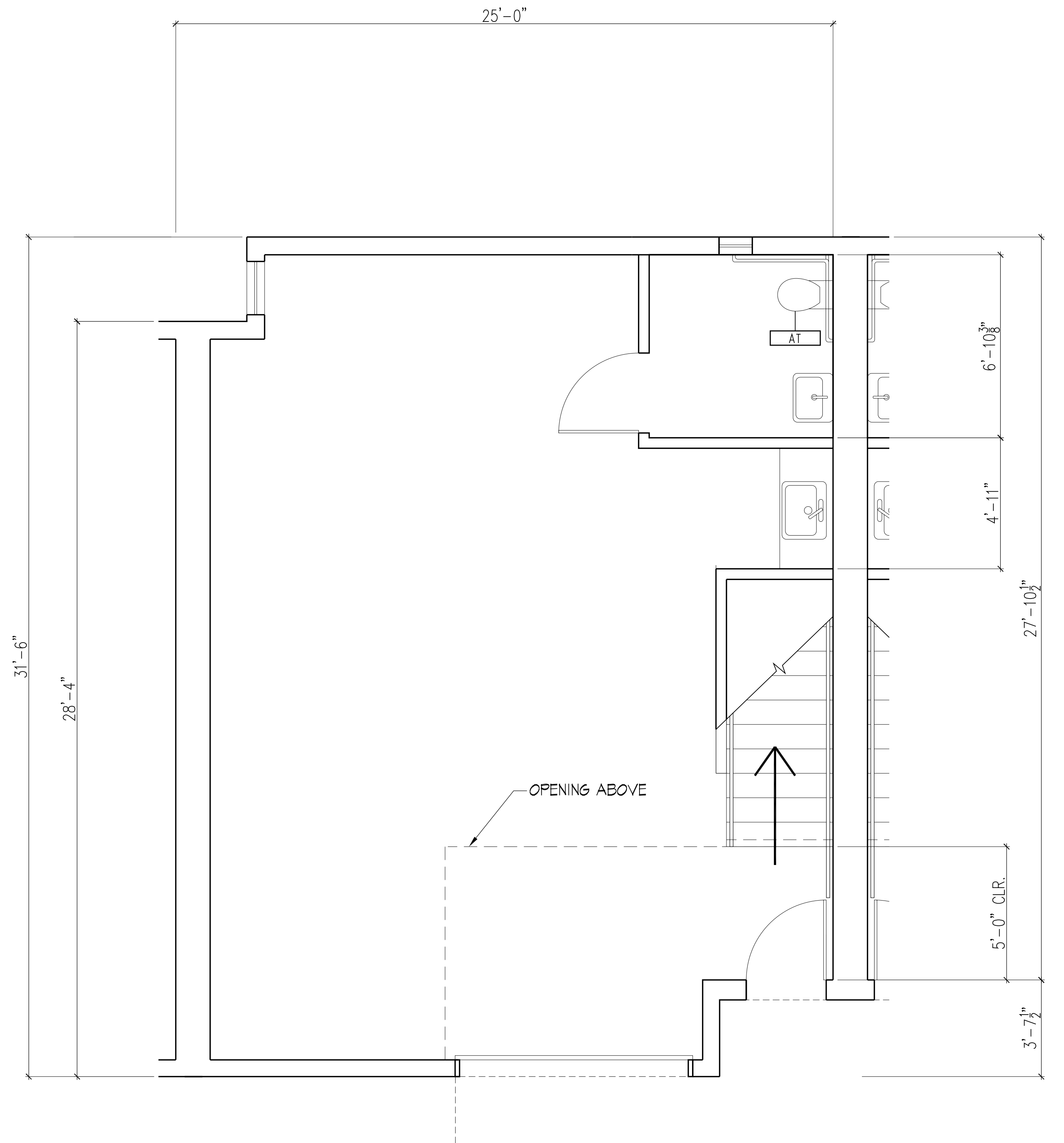
1 Unit C 1st Floor Plan 3/8" = 1'-0"
