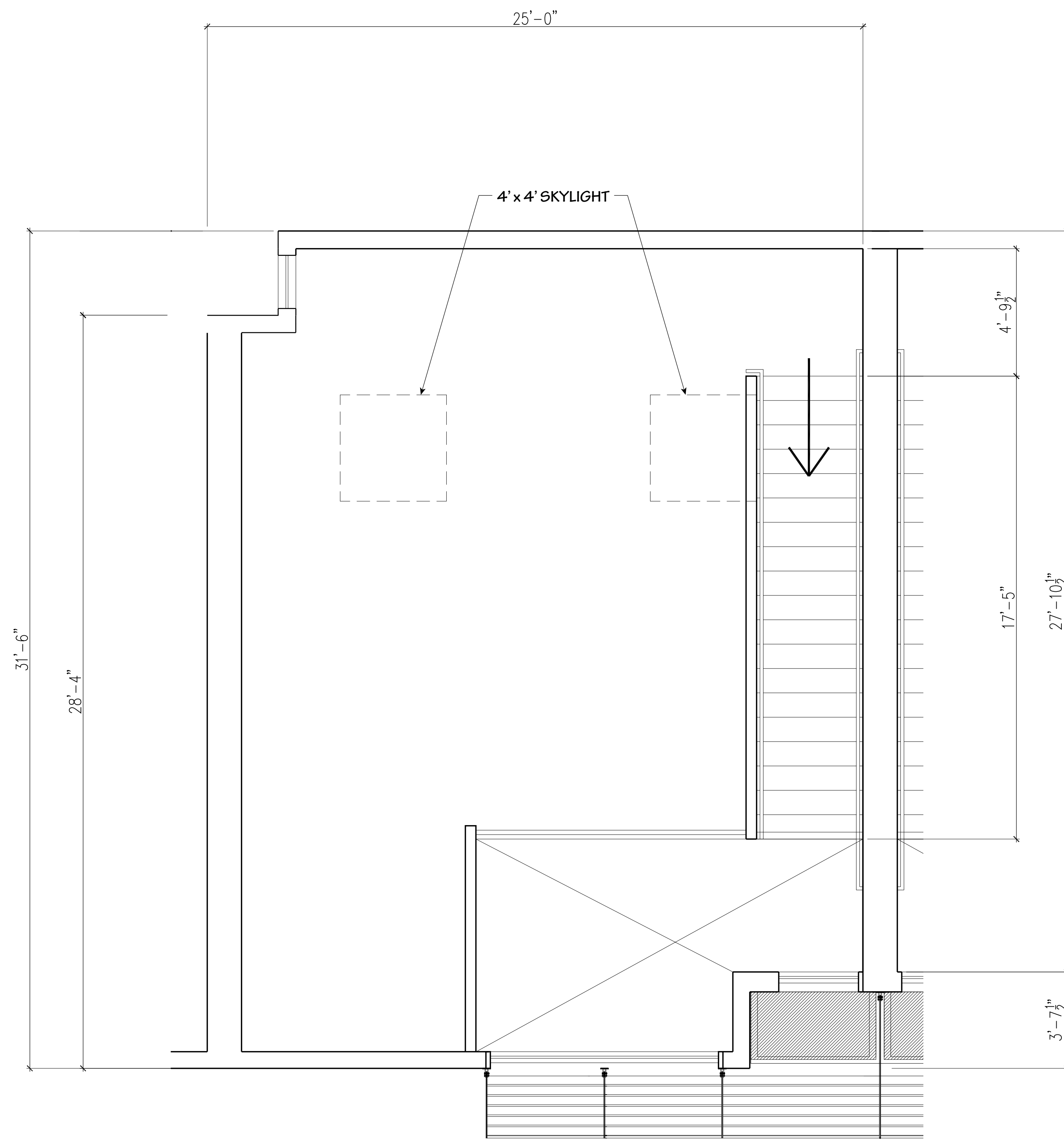
2 Unit E 2nd Floor Plan 3/8" = 1'-0"
